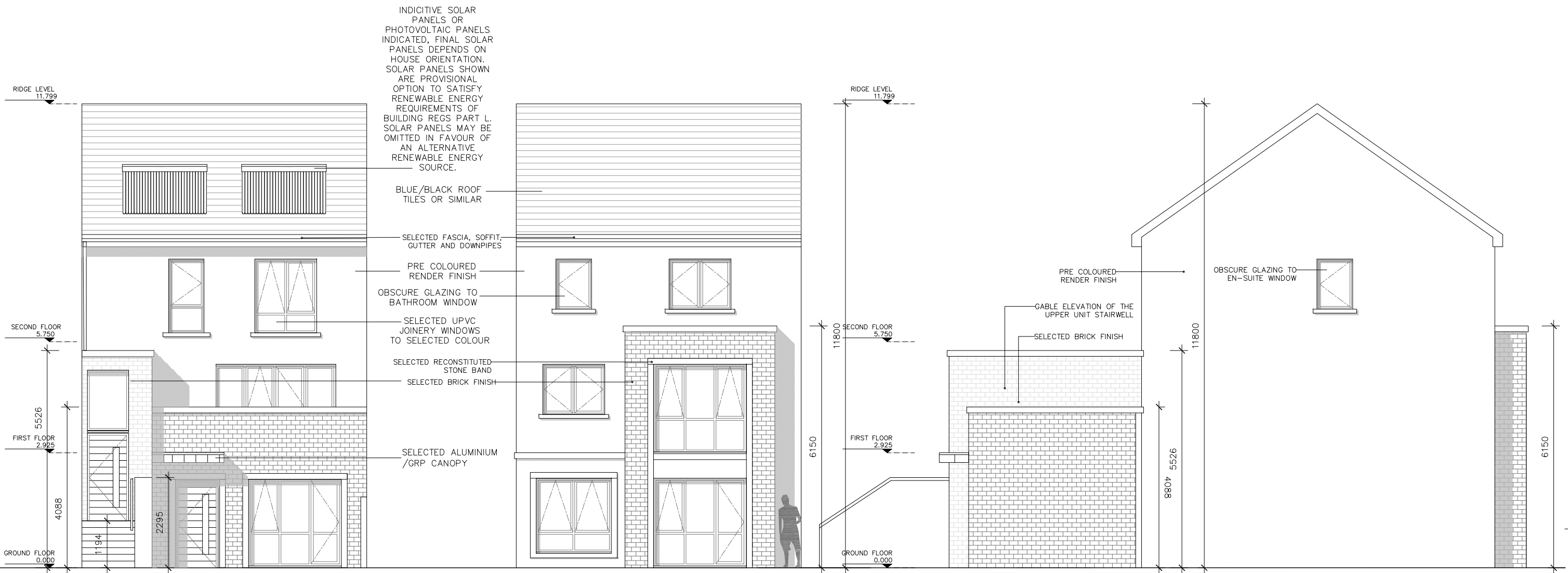
01 Front Elevation PA-D-300 1:100
